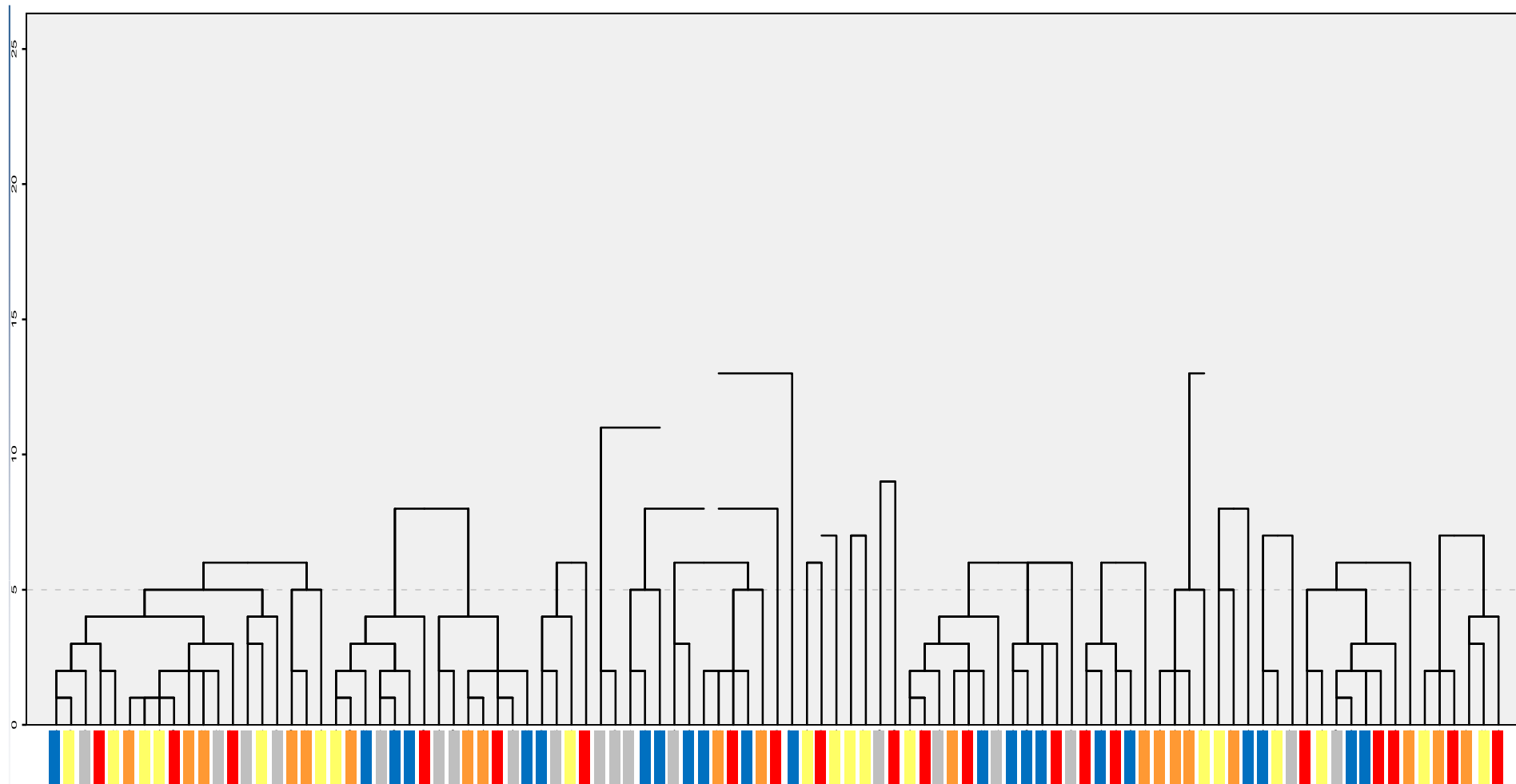
Dendrogram using Average Linkage (Between Groups): Rescaled Distance Cluster Combine
